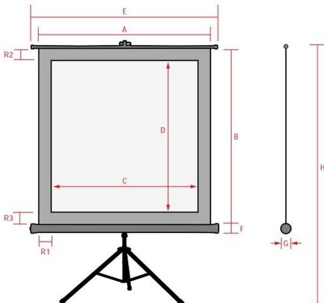
Tripod CrystalLine - Technical data (all dimensions in cm)
